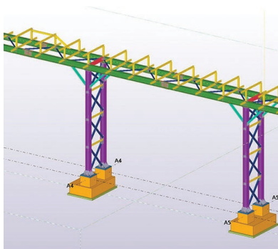
2019 SOVRAPPASSO PIPERACK ORION ENGINEERED CARBONS RAVENNA
